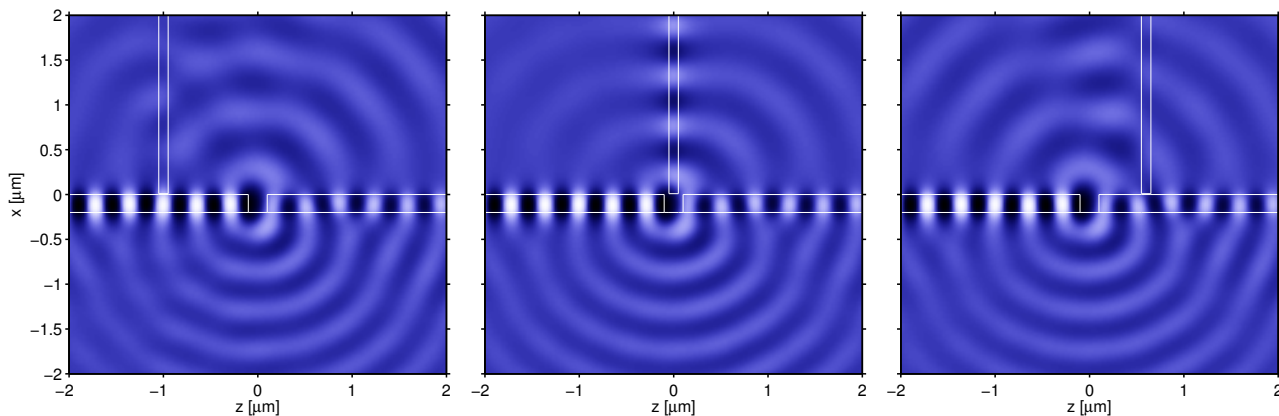
Snapshots of the electric field E_y for TE light propagation through the 2D microscope model, for three different probe positions. A slab waveguide (thickness 0.2 \mu\text{m} , refractive indices: 1.45, 2.0, 1.0) with a 0.2 \mu\text{m} hole forms the sample. The vertical core (width 0.1 \mu\text{m} , refractive index 1.5) represents the fiber tip. The sample is illuminated from the left by the fundamental mode (vacuum wavelength 0.633 \mu\text{m} ) of the horizontal channel. QUEP simulation with 80 \times 80 expansion terms on a 6 \mu\text{m} \times 6 \mu\text{m} computational window.
