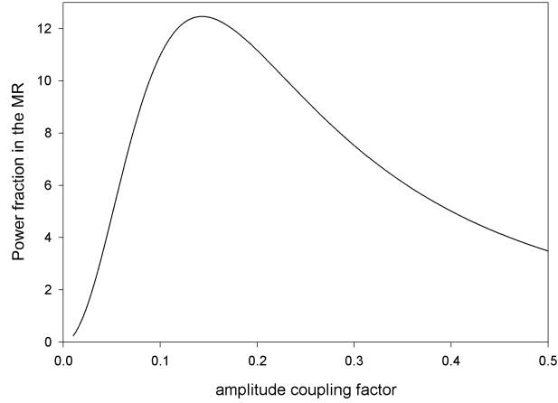
Figure 2: Power inside the Cylindrical microresonator as a function of the coupling coefficients
