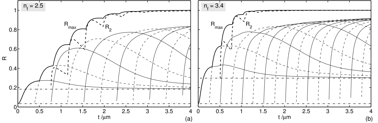
Figure 5: Mode reflectivities R versus the film thickness t , for facet configurations according to Figure 1 with film refractive indices n_f = 2.5 (a) and n_f = 3.4 (b). The thin curves indicate the reflectivities of individual modes, where continuous and dashed lines correspond to even respectively odd input fields. The thicker continuous curve marks the highest reflectivity level R_{\text{max}} that can be reached by any incoming guided field superposition, the dashed line R_2 is meant for a bimodal input with relative amplitudes according to Eq. (4). Horizontal lines are the reflectivities predicted by the Fresnel equations for perpendicular incidence of plane waves on dielectric interfaces with refractive indices n_f|n_a (upper line) and n_s|n_a (lower line).
