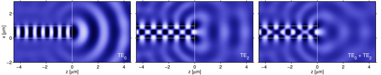
Figure 7: Electric field patterns for a facet excitation by low order modes, the fundamental field (left), the second order mode (center), and the superposition of the two that leads to the maximum guided reflected power (right); here the relative amplitude does not satisfy Eq. (4). The configuration is one of the structures of Figure 5(a): n_f = 2.5 , t = 1.0 \mu\text{m} .
