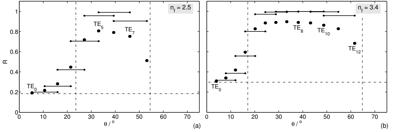
Figure 3: Modal reflectivities R versus the (discrete) mode angle, for a facet according to Figure 1 with waveguide thickness t = 3.15 \mu\text{m} and film refractive indices n_f = 2.5 (a) and n_f = 3.4 (b). Dots denote the relative guided power |r_{mm}|^2 that is reflected if a single guided field with the proper mode angle is launched. Horizontal bars mark the guided reflection, if the facet is excited by a superposition Eq. (4) of the two modes with angles at the bar end points. The vertical lines correspond to the critical incidence angles \theta_{crit} and the maximum mode angles \theta_{max} as given in the caption of Figure 2.
