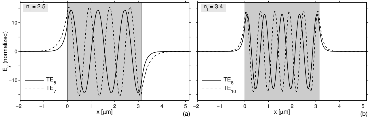
Figure 6: Normalized guided mode profiles that constitute the basis for the high reflection configurations of Figures 3, 4. The mode angles associated with these profiles are 33.0^\circ ( TE_5 ) and 46.0^\circ ( TE_7 ) for the lower index core n_f = 2.5 (a), and 38.1^\circ ( TE_8 ) and 48.7^\circ ( TE_{10} ) for the high contrast configuration n_f = 3.4 (b). The waveguide thickness is t = 3.15 \mu\text{m} in both cases.
