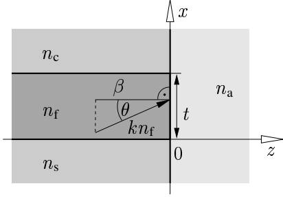
Figure 1: The waveguide facet. z and x denote the Cartesian coordinate axes parallel and perpendicular to the film plane. The geometry is specified in terms of the film thickness t and the refractive indices n_s , n_f , n_c , and n_a of the substrate, the film, the cladding material, and the medium adjacent to the facet. A mode angle \theta is assigned to each guided field with propagation constant \beta .
