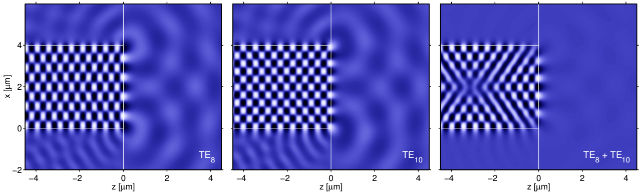
Figure 9: Analogue to Figure 4(b), for a nonsymmetric waveguide with thickness t = 4.0 \mu\text{m} , film refractive index n_f = 3.4 and a substrate refractive index of n_s = 2.4 . The reflectivity values observed in the three simulations are |r_{88}|^2 = 0.91 , |r_{1010}|^2 = 0.90 , R_2 > 0.998 .
