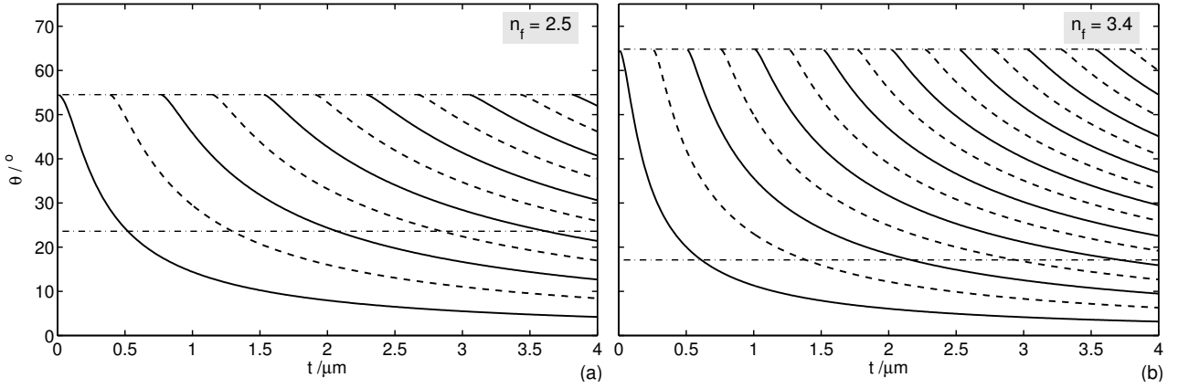
Figure 2: Angles \theta associated with guided mode propagation constants versus the waveguide thickness, for symmetrical planar waveguides as specified by Figure 1 with core refractive indices n_f = 2.5 (a) and n_f = 3.4 (b); see the text for other parameter values. The lower horizontal lines indicate the critical incidence angles \theta_{\text{crit}} = 23.6^\circ (a) and \theta_{\text{crit}} = 17.1^\circ (b) for total plane wave reflection at an interface between two media with refractive indices n_f and n_a , the upper lines are placed at the cutoff angles \theta_{\text{max}} = 54.5^\circ (a) and \theta_{\text{max}} = 64.8^\circ (b) for guided wave propagation in the ended waveguides.
