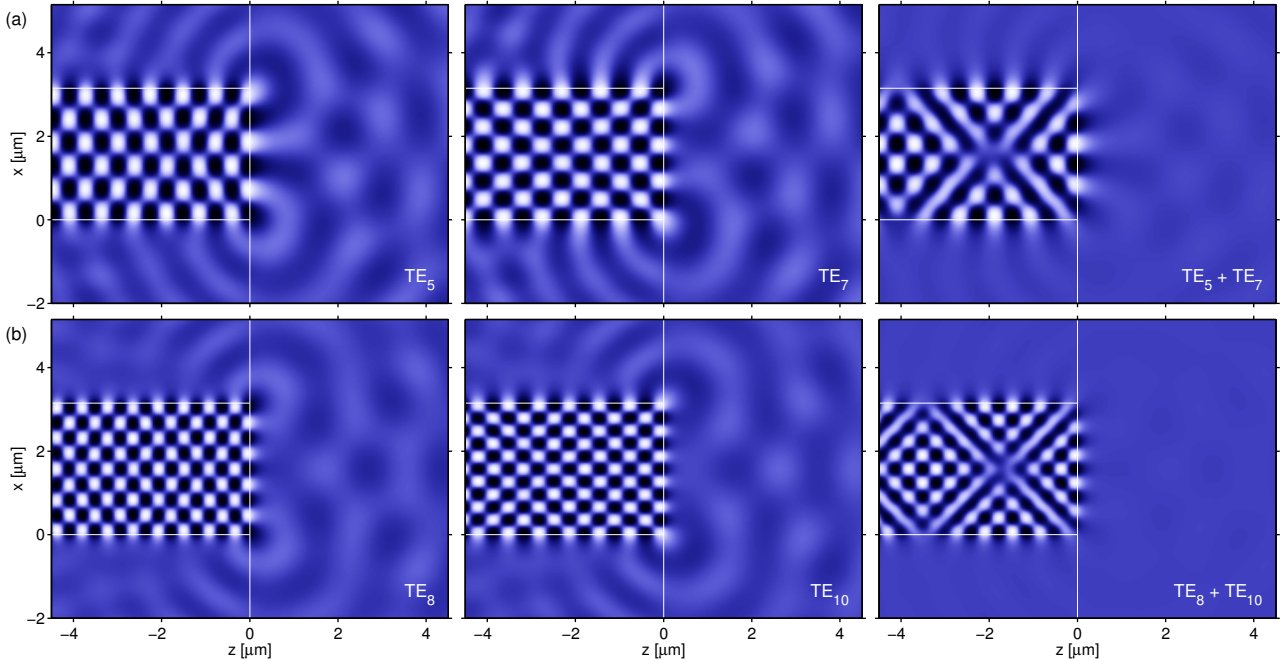
Figure 4: Snapshots of the electric field \mathcal{E}_y at selected times for facets as sketched in Figure 1, t = 3.15 \mu\text{m} , n_f = 2.5 (a, top row) and n_f = 3.4 (b, bottom row). For the lower index core (a), the 5th and 7th order modes are first launched separately (left and center), then simultaneously with a specific relative amplitude according to Eq. (4) (right). For the higher index film (b), the 8th and 10th order modes and their superposition were considered. White and black regions mean positive and negative field strength, the gray background (the surrounding in the lower right inset) indicates the zero level. The reflectivities corresponding to these plots are |r_{55}|^2 = 0.81 , |r_{77}|^2 = 0.75 , R_2 > 0.990 (a), and |r_{88}|^2 = 0.89 , |r_{1010}|^2 = 0.86 , R_2 > 0.998 (b).
