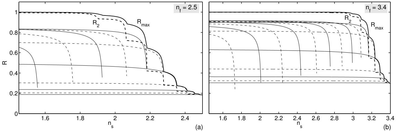
Figure 8: Mode reflectivities R versus the substrate refractive index n_s , for facets of nonsymmetric waveguides according to Figure 1 with a core thickness t = 4.0 \mu\text{m} and film refractive indices n_f = 2.5 (a) and n_f = 3.4 (b). See the caption of Figure 5 for the interpretation of the line styles.
